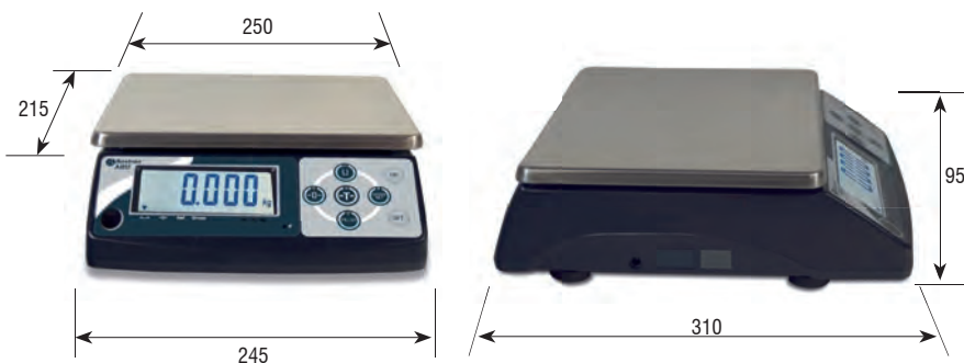
Dimensions (mm)
